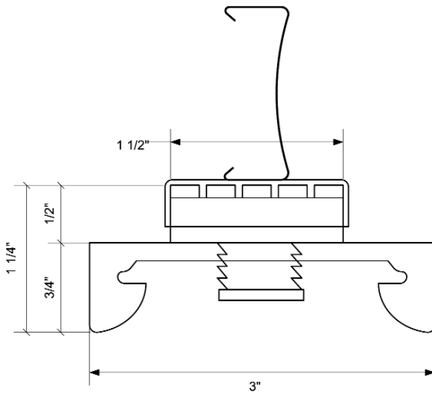
PROFILE VIEW
