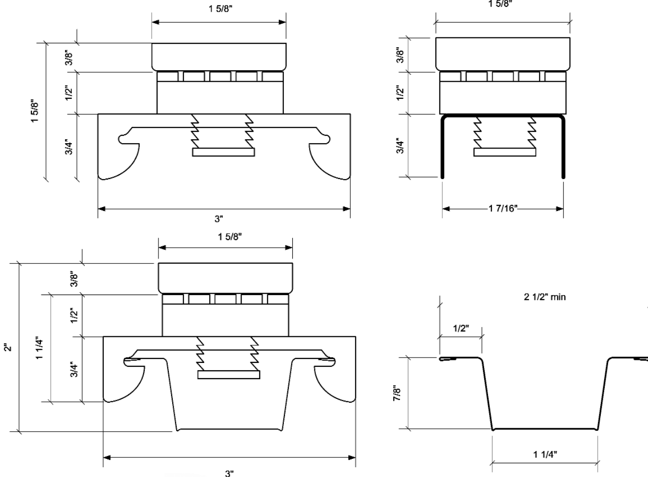
END VIEW
